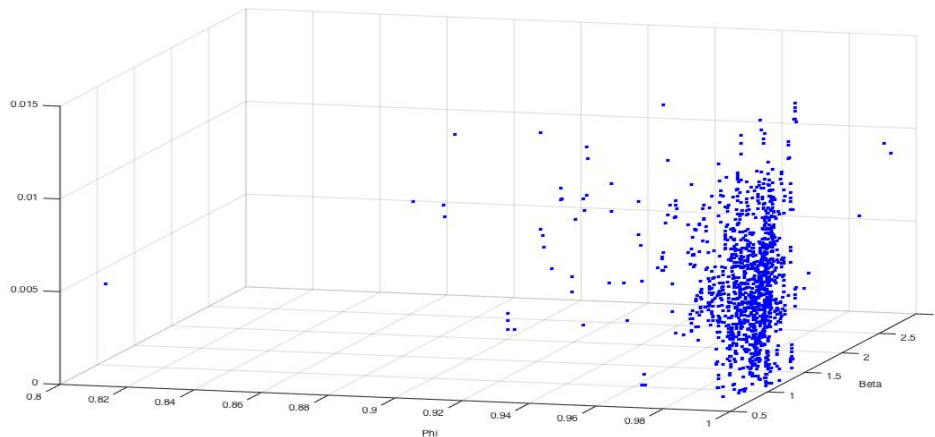
Figure 2: Stationary desirable mutual funds 3D-Plot
